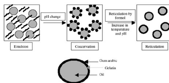
Figure 1. Principle of the complex coacervation method.
