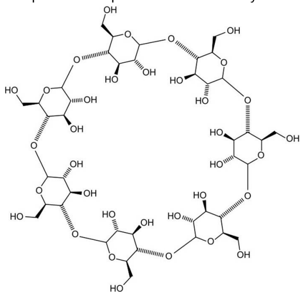
Figure 2. Structure of \beta -cyclodextrin molecules.
