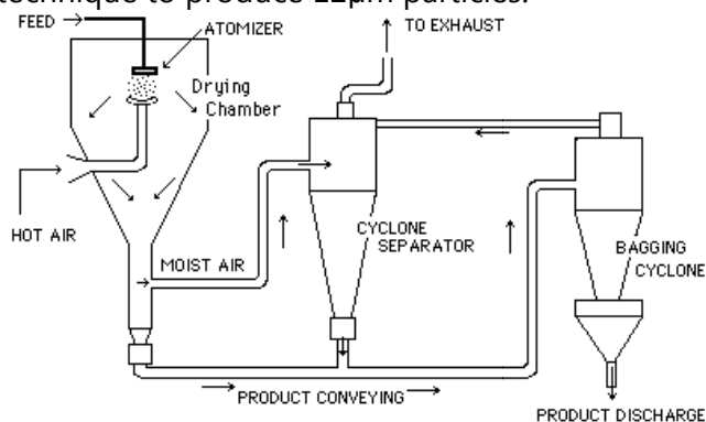
Figure 4. Spray drying process.
